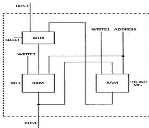
Fig. 8. The internal organization of the MFs block.
