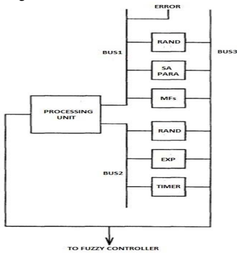
Fig. 7. The data-path for the SA-tuning mechanism.
