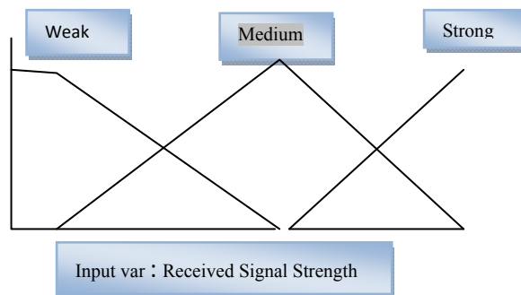
Fig. 5. Membership functions of received signal strength (RSS)
