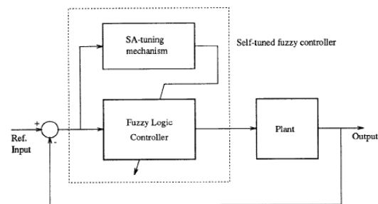
Fig. 1. A closed-loop self-tuned fuzzy control arrangement.
