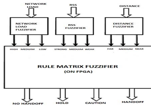
Fig. 3. Fuzzy controller on FPGA
