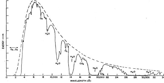
FIGURE 2. Spectral distribution of sunlight arriving at earth's surface.
