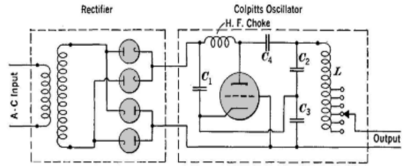
Figure 11. Fundamental Circuit With Colpitts Oscillator for Converting Low-Frequency Power to High-Frequency Power
