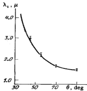
Figure 10. Dependence of the wavelength of the converted infrared radiation \lambda_i on the phase-matching angle \theta .
