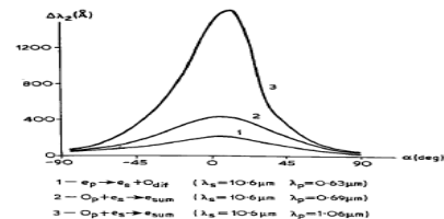
Figure 8. The dependence of the conversion spectral bandwidth on the angle \alpha between the pump and signal wave directions
